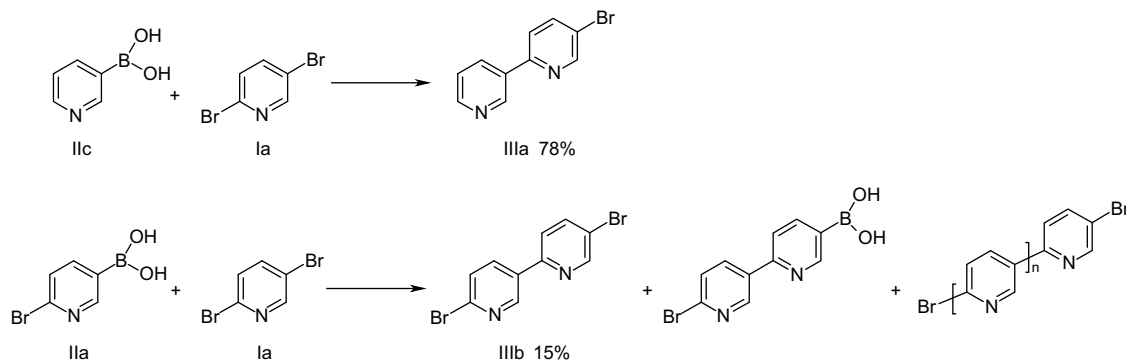
Scheme 3. Synthesis of halopyridinylboronic acids IIIa and IIIb .
