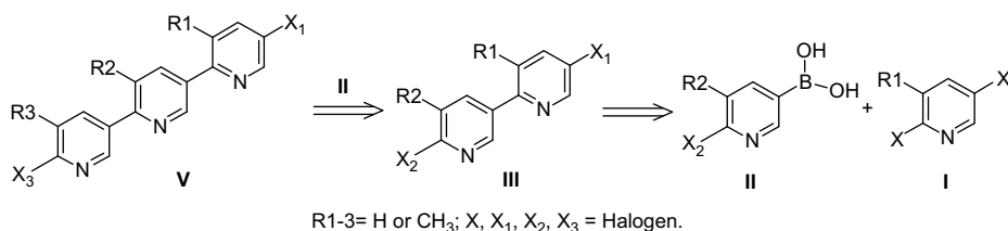
Scheme 1. Retrosynthetic aspect.
